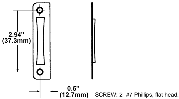
FIG.5 IN-LINE STRIKE HOUSING 299-105
