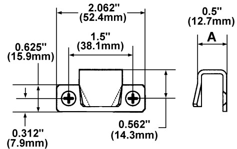
FIG.4 U-SHAPE KEEPER 299-107
