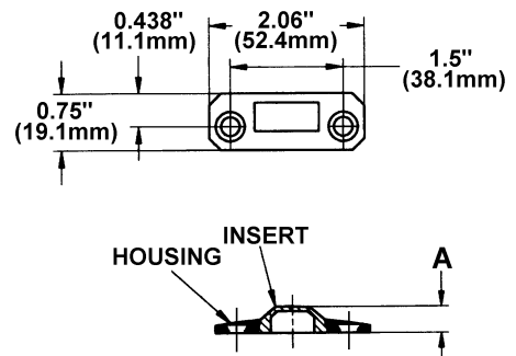
FIG.6 OFFSET STRIKE HOUSING 299-106
