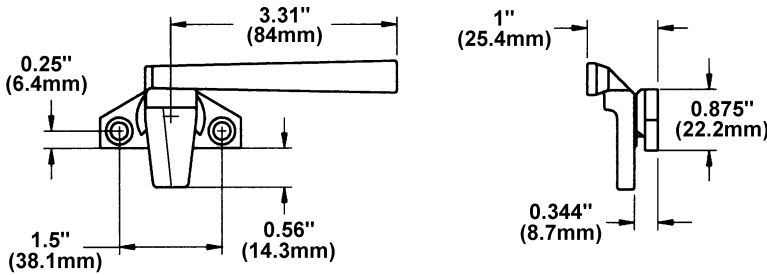
FIG.1 DUAL SIDED CAM HANDLE (offset base) RH:225-029 & LH:225-028
