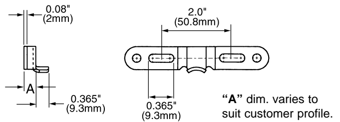
FIG. 3 STAINLESS STEEL KEEPERS
