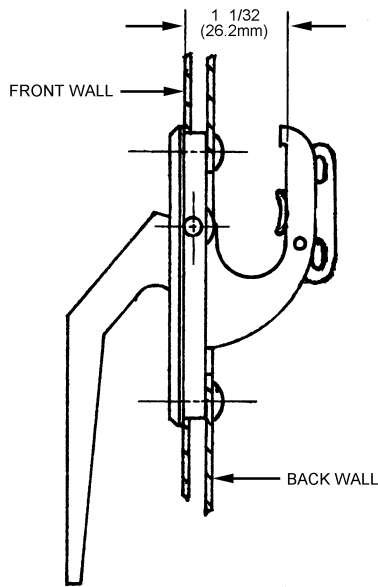
FIG. 2 PROFILE CUT-OUT FOR HANDLE
