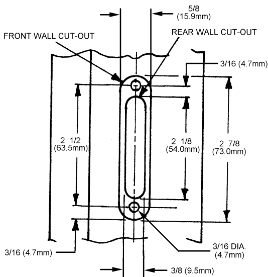
FIG. 2 PROFILE CUT-OUT FOR HANDLE
