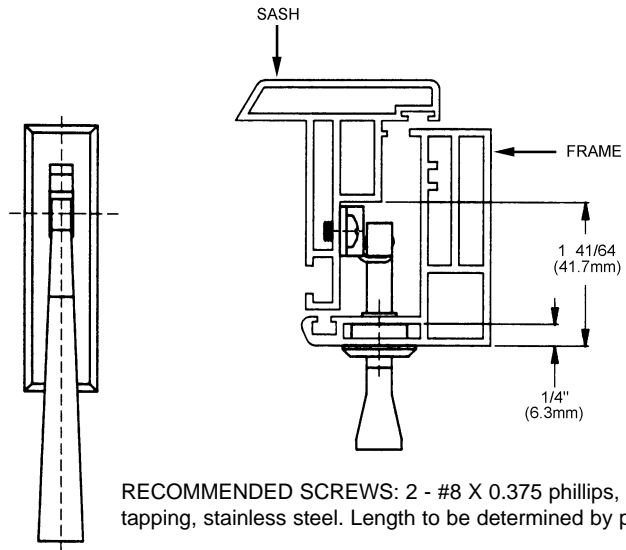
FIG. 3 STAINLESS STEEL KEEPERS
