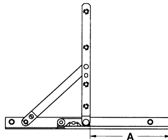
FIG. 2 HINGE OPENING DIAGRAM
